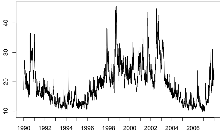
Figure 2.1: VIX index 1.1.1990 - 31.12.2007
