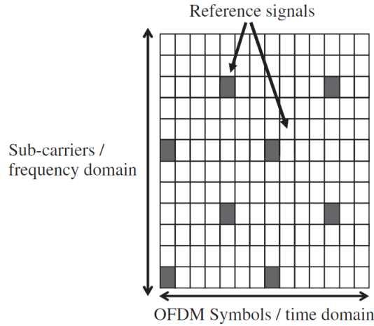
Figure 8: Reference signal mapping principle [3]
