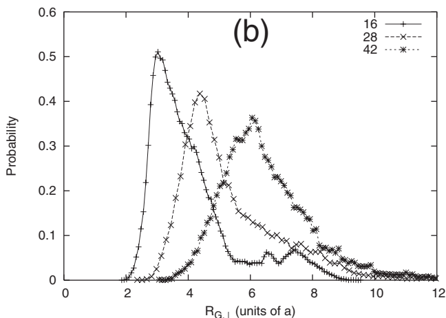
FIG. 3. The distributions of the two components of the radius of gyration: (a) in the direction parallel to gravity, and (b) in the direction perpendicular to gravity. The chain lengths are indicated in the figures.
