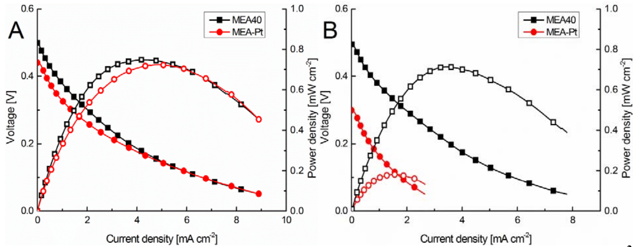
Fig. 6. The DMFC performance of the N-FWCNT cathode (MEA40, 2.3 mg (N-FWCNT) cm -2 ) and Pt/C cathode (MEA-Pt, 0.5 mg (Pt) cm -2 ). A) O 2 , B) air as oxidant. The full symbols refer to voltage curves and open symbols to power curves.
