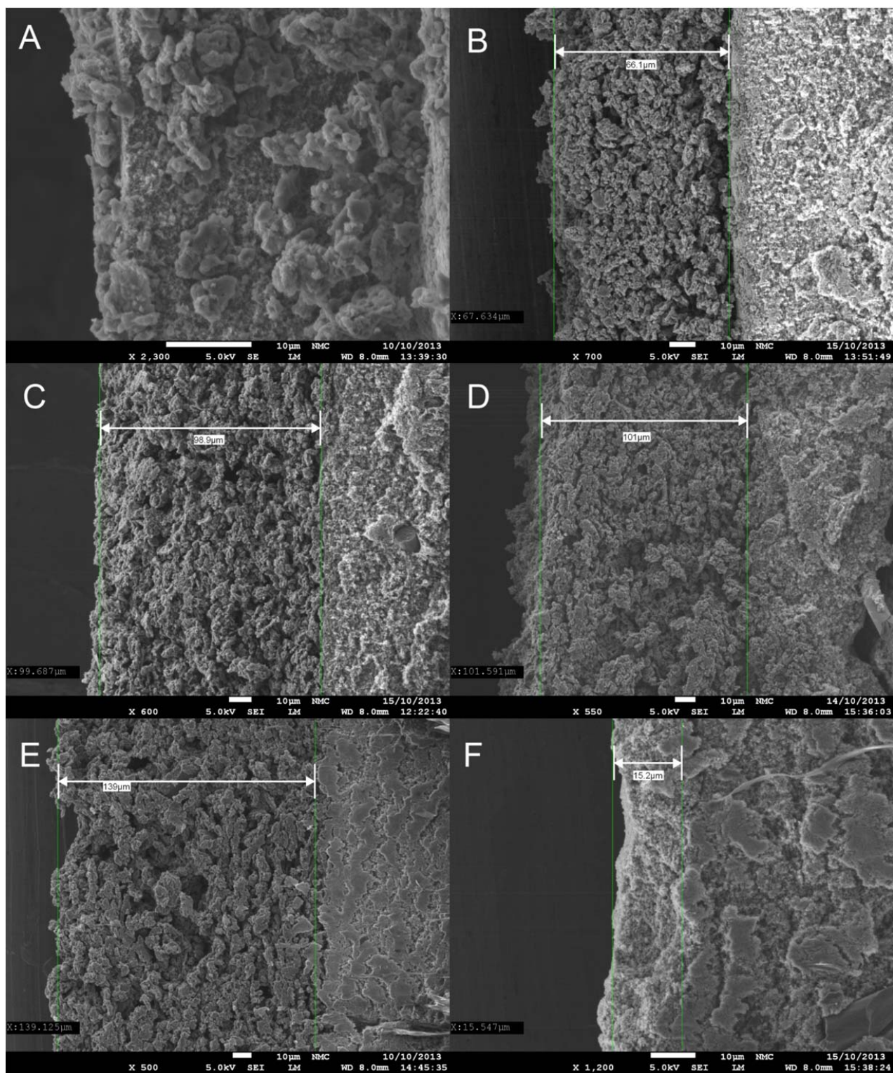
Fig. 7. SEM images of the cross-sections of the cathode catalyst layers. A) MEA20, B) MEA30, C) MEA40, D) MEA50, E) MEA60, F) MEA-Pt
