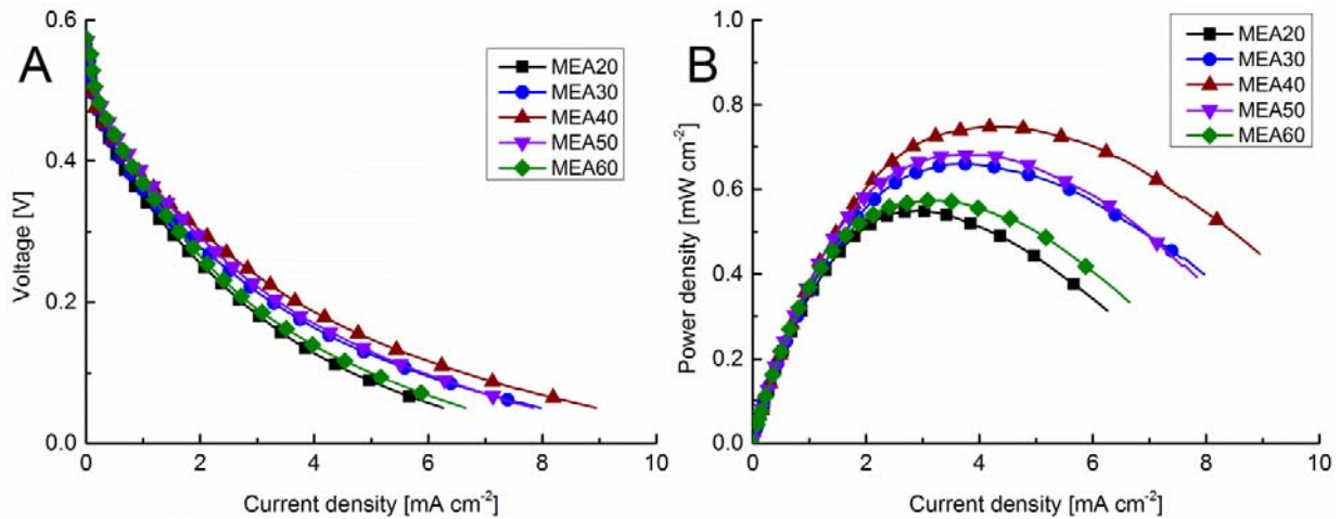
Fig. 2. The DMFC performance with the different FAA3 ionomer contents in the N-FWCNT cathode catalyst layer. The oxidant is O 2 . A) voltage and B) power density curves.
