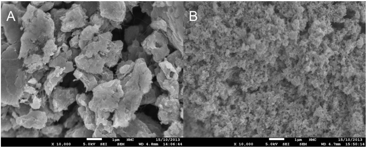
Fig. 8. Higher magnification (10000x) of the cathode catalyst layers of A) MEA30 (31 wt% FAA3) and B) MEA-Pt (29 wt% FAA3).
