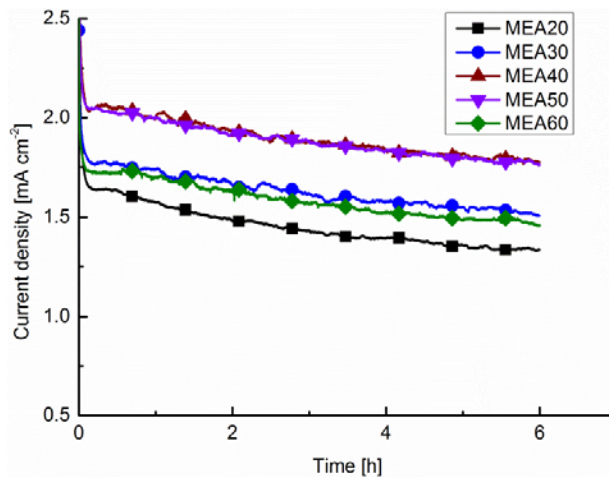
Fig. 5. 6-hour constant voltage measurements at 0.2 V in DMFC.
