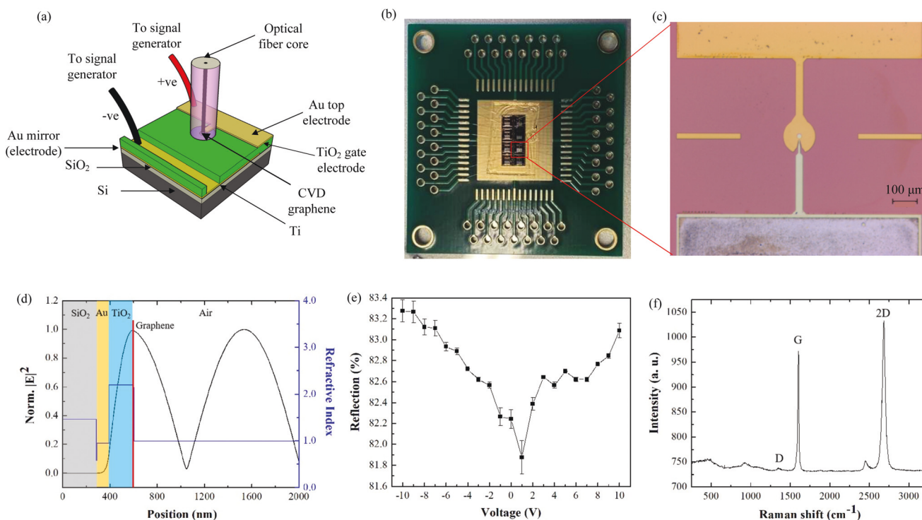
Fig. 1 (a) Schematic illustration of the fibre-integrated modulator structure. A parallel-plate capacitor is formed between graphene, titanium oxide (TiO 2 ), and the gold mirror/electrode. Note that the illustration is a not-to-scale drawing. (b) Image of the modulator array on a single chip fixed on a PCB. (c) Optical microscopy image of a single modulator with 5 \times objective magnification. (d) Normalized electric field intensity and refractive index distribution along the normal direction of the modulator. (e) Optical reflection as a function of the electrical voltage applied to the modulator. (f) Raman spectrum of the graphene utilized for the modulator.
