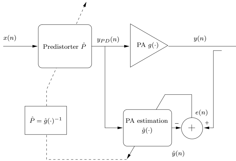
Figure 4.9: Predistorter implementation using direct learning structure
