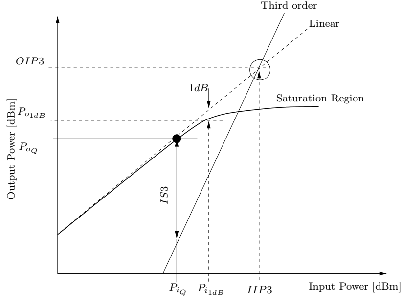
Figure 2.6: Illustration of input third-order intersection point (IIP3), output third order intersection point (OIP3), and 1dB compression point ( P_{i1dB}, P_{o1dB} ). IS3 denotes the third-order intermodulation suppression for a particular working point P_{iQ}, P_{oQ} .
