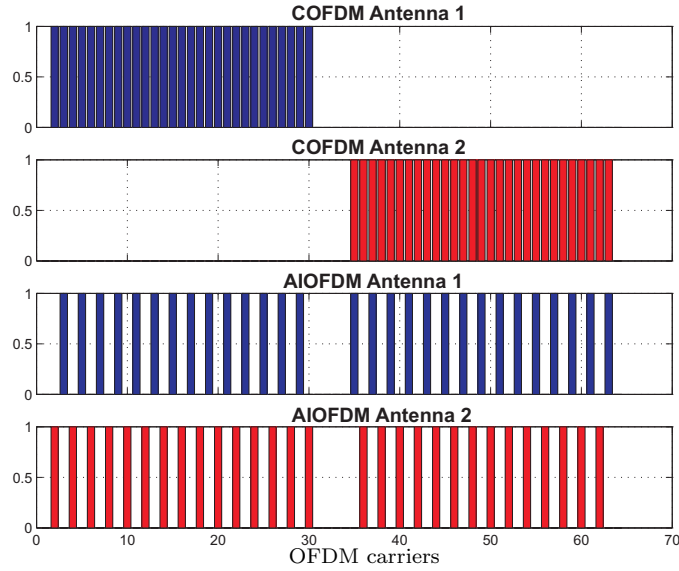
Figure 4.7: Carrier allocation for COFDM and AIOFDM for an OFDM system using N = 64 subcarriers and M = 2 antennas
