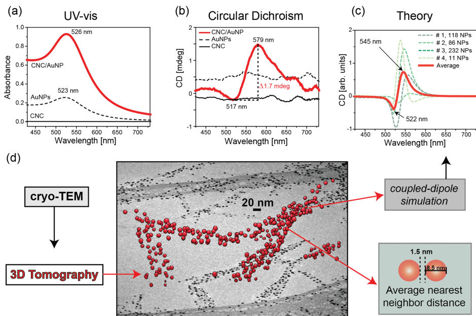
Figure 3. a) UV-vis and (b) CD spectra of CNCs, AuNPs (8.5 nm) and CNC/AuNP (8.5 nm) fibrillar superstructures. c) Simulated CD spectra for four different CNC/AuNP fibrillar superstructure tomograms (samples #1–4) taken from different positions, having different numbers of AuNPs. d) Example of cryo-ET reconstruction using 118 AuNPs (red color on top of gray-scale cryo-TEM image of the same assembly, sample #1, Supporting Information). The average nearest neighbor distance of 1.5 nm (sample #1).
