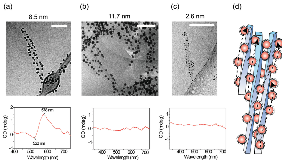
Figure 2. Cryo-TEM images and circular dichroism measurements upon electrostatic binding of AuNP onto CNC: AuNP core sizes: a) 8.5 \text{ nm} , b) 11.7 \text{ nm} , and c) 2.6 \text{ nm} . Scale bars: 100 nm. d) The proposed scheme CNC/AuNP ( 8.5 \text{ nm} ) fibrillar superstructures, where a few anionic CNC rods with their internal right-handed chiral twisting bind positively charged AuNPs. The right-handed twisting of CNCs induces a right-handed component in the AuNP packing.
