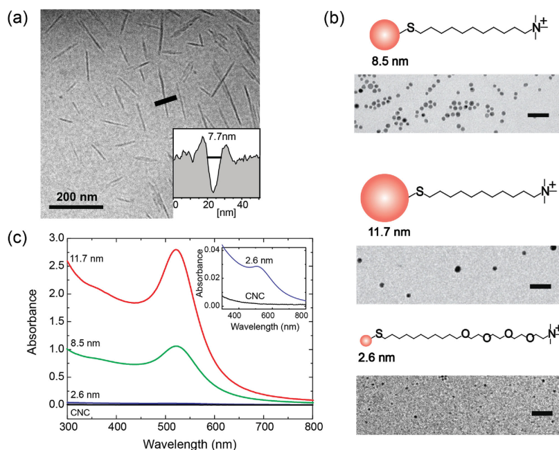
Figure 1. Starting materials. a) Cryo-TEM of pristine CNCs ( 5 \text{ mg mL}^{-1} ). b) AuNPs showing the cationic ligands, the metal core sizes, and cryo-TEM images. Scale bars: 50 nm. c) UV-vis spectra of the CNCs and three different cationic AuNPs normalized to the same AuNP concentration.
