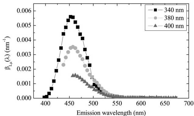
Fig. 1. Bispectral luminescent radiance factors for three excitation wavelengths measured in 0°/10° geometry.
