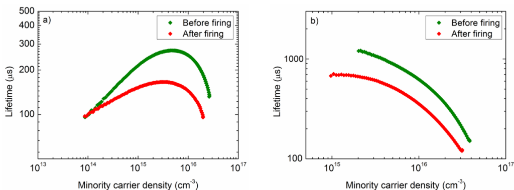
Fig. 5. Lifetime values as a function of minority carrier density before and after firing (~3 s, 800 °C) in (a) p-type CZ-Si and (b) n-type CZ-Si measured with QSSPC. ALD1 reactant set (TMA + O 3 ) was used in the Al 2 O 3 deposition. Annealing for 30 minutes at 450 °C in N 2 was done before the firing step.
