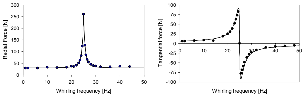
Fig. 5. The total force as a function of the whirling frequency.
