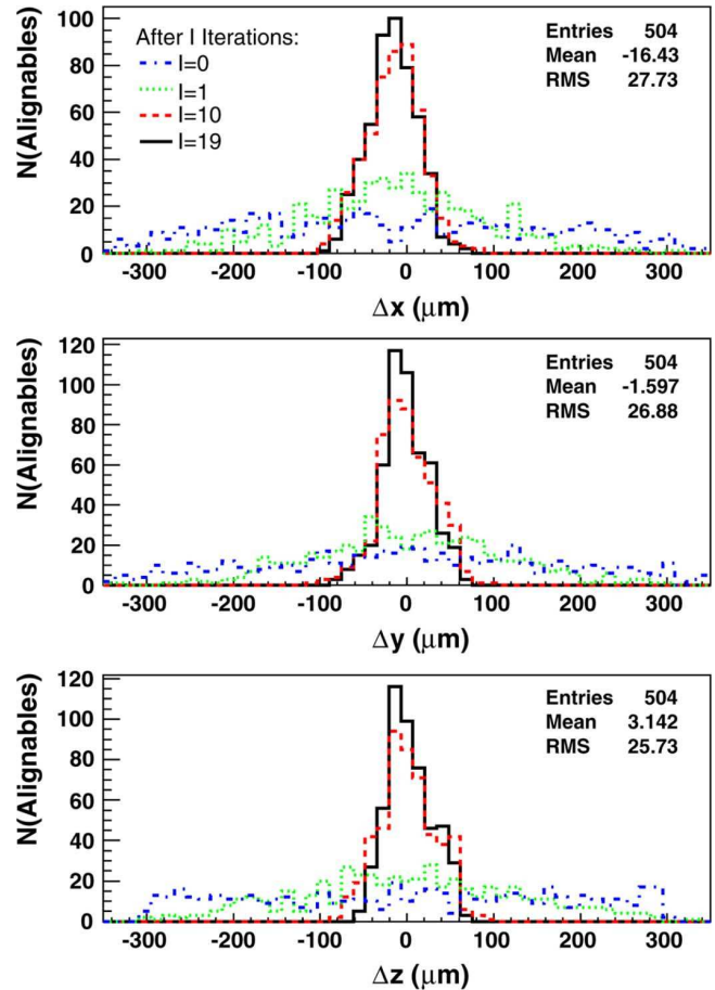
Fig. 2. Residual distributions of alignment of 504 pixel barrel modules. The residuals in global coordinates are shown for the initial misalignment (iteration 0) and after 1, 10, and 19 iterations. The statistical parameters refer to the iteration 19.
