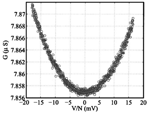
FIG. 3. Measured data (○) of dynamic conductance G=dI/dV plotted vs voltage over one junction. Fitting a parabola (solid line) gives, using the Simmons model, an effective barrier width of d=12 Å and a barrier height of \phi=3 eV. This measurement was performed at T=77 K. The measurement at 4 K gave almost identical results apart from the Coulomb blockade feature around zero bias.
