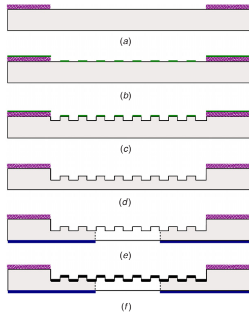
Figure 2. Process flow for the preparation of the silicon chip: pattern the SiO 2 to define the flowfield area (a), pattern the photoresist mask for the flowfield channels (b), RIE of flowfield channels (c), RIE to sink the flowfield (d), backside gas inlet etch through Al mask (e) and black silicon formation and metallization (f).
