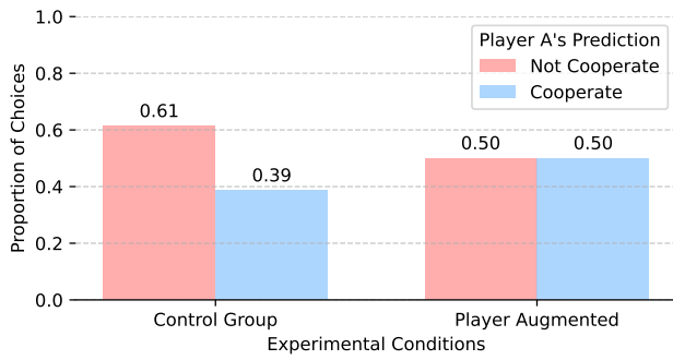
(a) Proportion of Player A's Prediction by Condition
