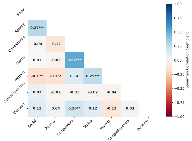
(b) Spearman Correlation Matrix (Prisoner's Dilemma).
