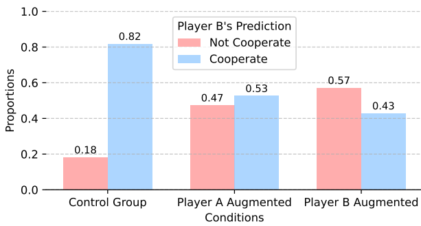
(b) Proportion of Player B's Prediction by Condition.
