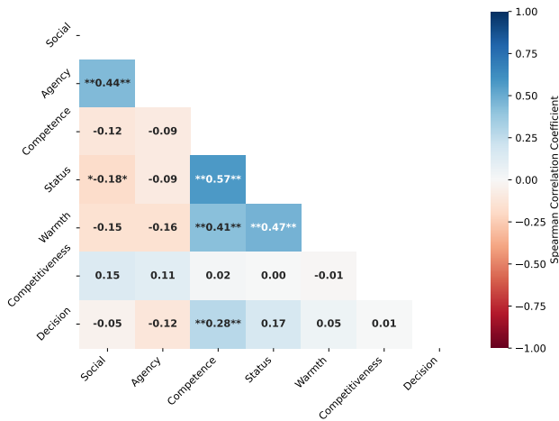
(a) Spearman Correlation Matrix (Trust Game).
