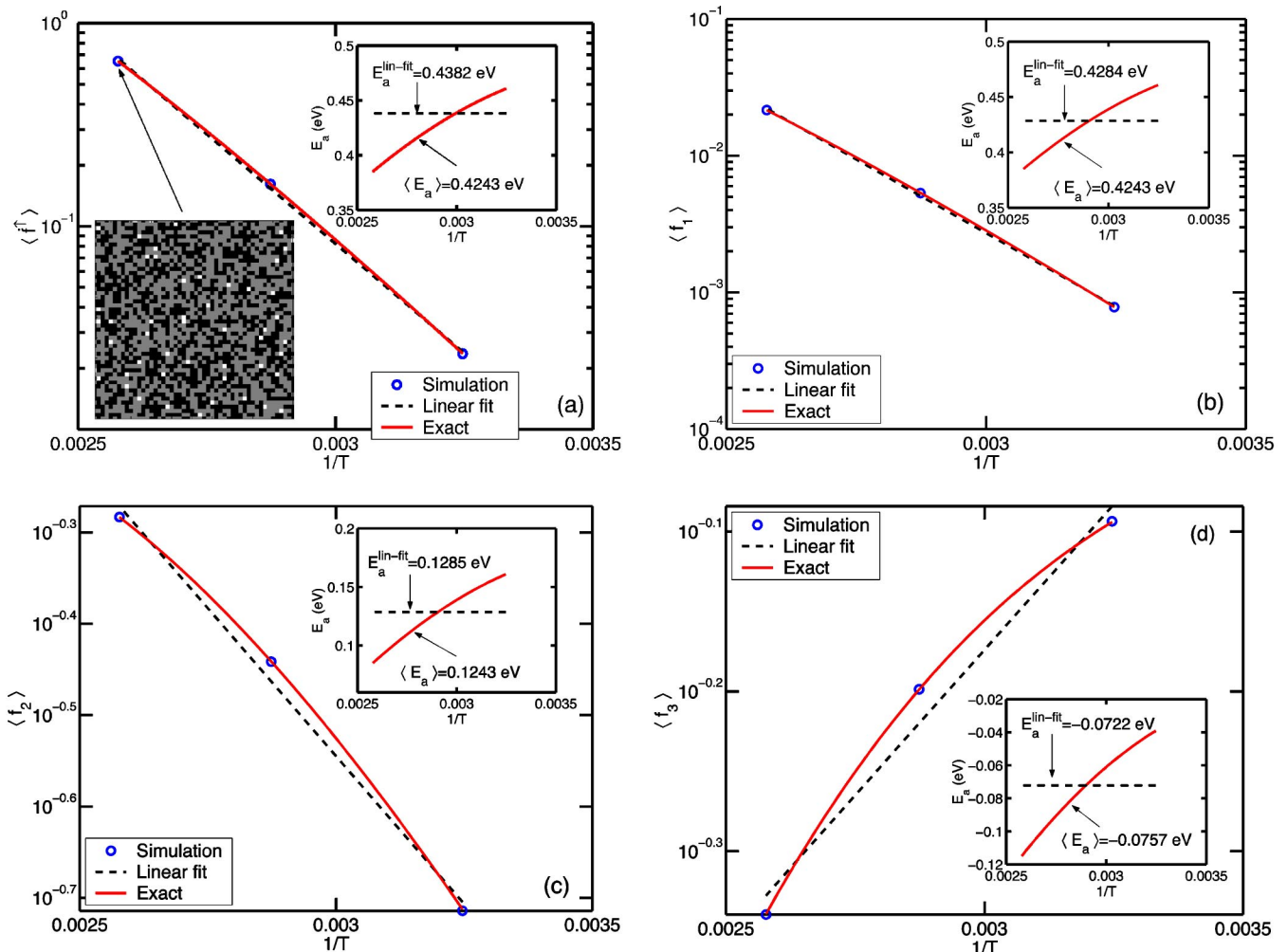
FIG. 2. (Color online) Arrhenius plot of (a) the rate of removal of particles \langle f^{\uparrow} \rangle and the surface fractions (b) \langle f_1 \rangle , (c) \langle f_2 \rangle , and (d) \langle f_3 \rangle for case D.
