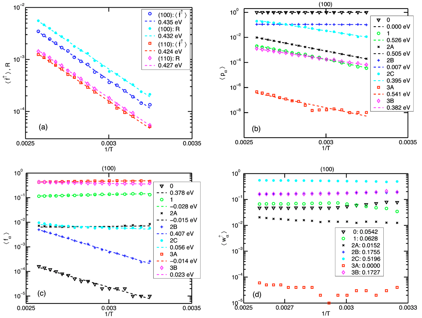
FIG. 8. (Color online) (a) Etch rate R and rate of removal of particles \langle f^\dagger \rangle for (100) and (110). (b),(c) Determination of the activation energies E_{\langle p_\alpha \rangle} and E_{\langle f_\alpha \rangle} ( \alpha=0,1,2A, \dots, 3B ) for (100). (d) Temperature dependence of the normalized fractions of removed particles \langle w_\alpha^\dagger \rangle .
