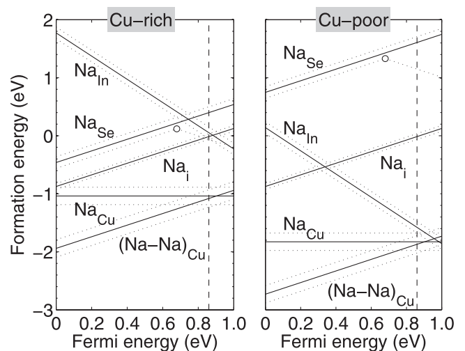
FIG. 1. Formation energies of sodium-related point defects and (\text{Na}-\text{Na})_{\text{Cu}} dumbbell in CIS as a function of Fermi energy. At the Cu-rich limit, the corresponding chemical potentials for In and Se are \Delta\mu_{\text{In}} = 0 eV and \Delta\mu_{\text{Se}} = -1.21 eV. At the Cu-poor limit, the chemical potentials are \Delta\mu_{\text{Cu}} = -0.79 eV, \Delta\mu_{\text{In}} = -1.63 eV, and \Delta\mu_{\text{Se}} = 0 eV. The chemical potential for sodium is that of metallic bcc sodium. The dotted lines give error estimates for the formation energies at each Fermi level position. The dashed line marks the band gap obtained with HSE06.
