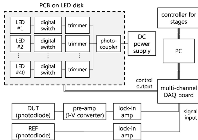
Figure 6: Block diagram of the instrumentation [5].
