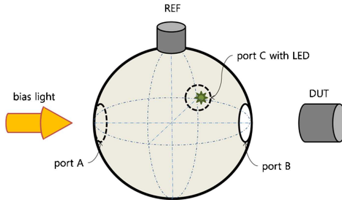
Figure 4: Detailed view of the integrating sphere [5].
