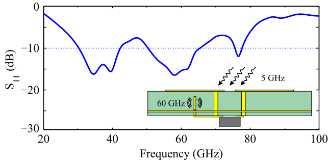
FIGURE 10. Amplitude of scattering parameter S_{11} for a monopole antenna of L_{\text{ant}} = 1.2 mm, at its 50 \Omega feed port marked with red color in the inset, which depicts the cross-sectional side-view of a unit cell for the metasurface-layer intercell communication channel modeling.
