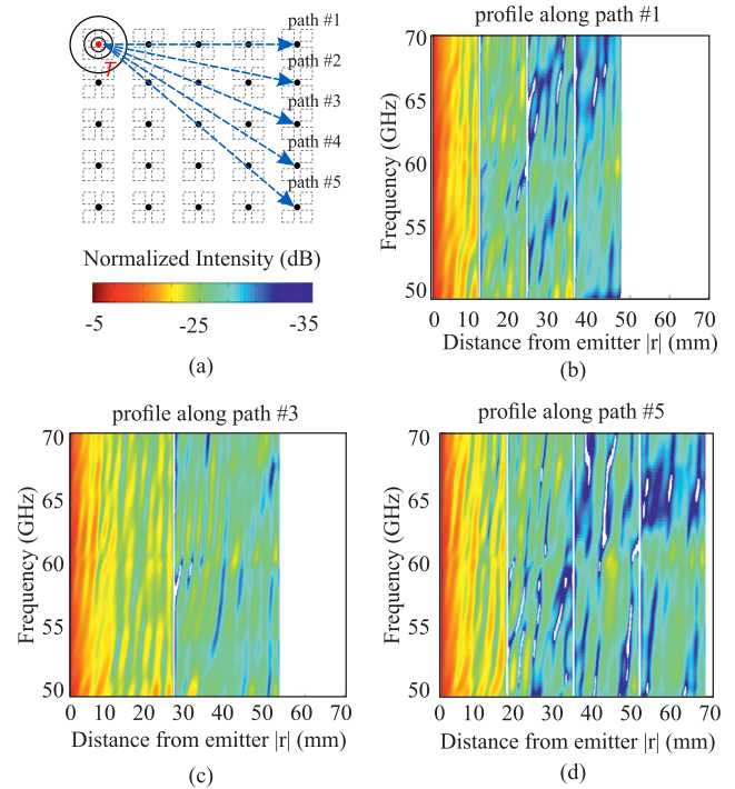
FIGURE 8. (a) A 5x5 grid of antennas where the emitter antenna is no. 1, in the corner. (b,c,d) Power transmission profiles, for frequency f = 50 to 70 GHz versus distance from the emitter; the colorbar refers to the power of the total field, emitted plus scattered, calculated along paths (b) #1, (c) #3 and (d) #5, as numbered in panel (a). These paths are selected so that all possible direction are included.
