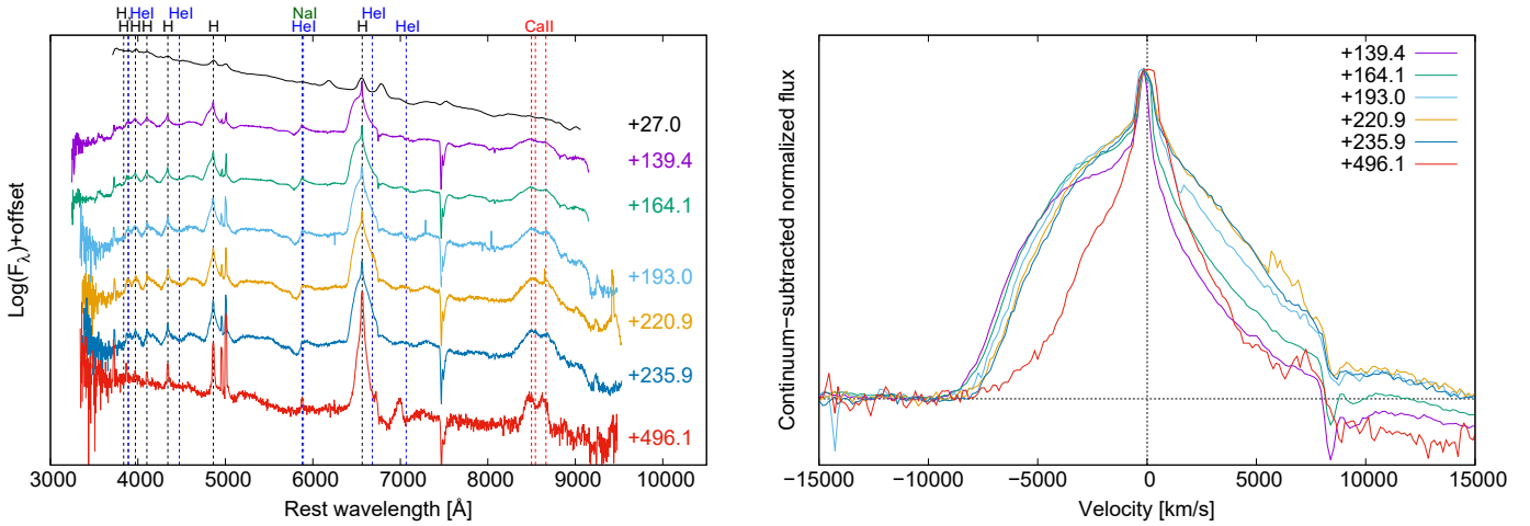
Fig. 3. Same as Fig. 2 but for SN 2021adxl. The continuum level is assumed to be a constant value and estimated from the averaged value from -15000 to -10000 \text{km s}^{-1} in the velocity space.
