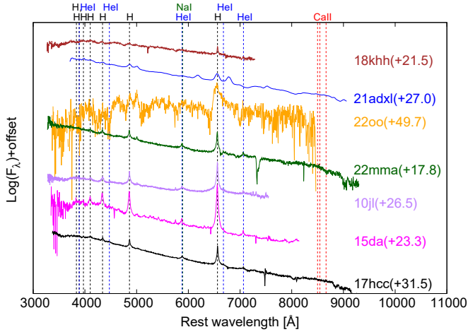
Fig. 6. Comparison of the early-phase spectra of the SNe in our sample. All spectra are corrected for extinction (see Section 2). The data for SNe 2010jl, 2015da, 2017hcc, and 2021adxl are taken from Smith et al. (2012), Tartaglia et al. (2020), Moran et al. (2023) and Brennan et al. (2024), respectively.
