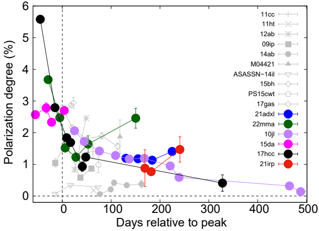
Fig. 12. Time evolution of the continuum polarization of the SNe in our sample with polarimetric data (colored points), compared with those of Type II SNe presented in Bilinski et al. (2024) (gray points). The R -band polarization is regarded as the continuum polarization for SNe 2021adxl and 2022mma. The data for SNe 2010jl, 2015da, 2017hcc, and 2021irp are taken from Bilinski et al. (2024, and references therein) and from Reynolds et al. (2025b).
