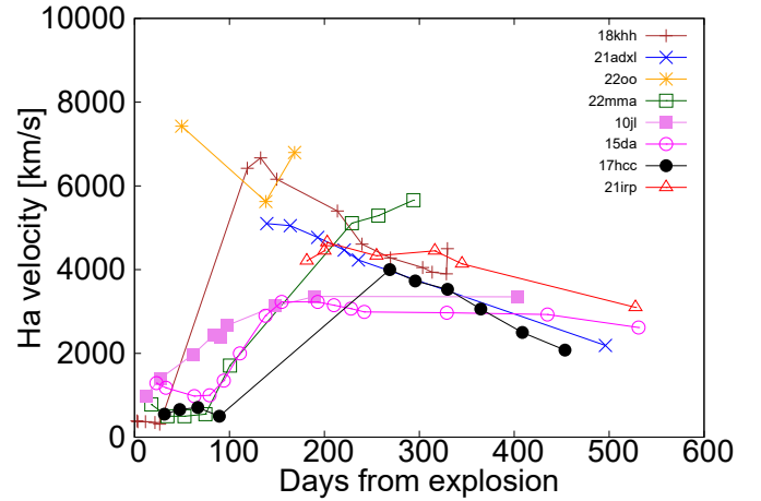
Fig. 8. Evolution of the H\alpha velocity. The velocity measurements for SNe 2010jl, 2015da, 2017hcc, and 2021irp are conducted using selected low-resolution spectra from Smith et al. (2012), Jencson et al. (2016), Tartaglia et al. (2020), Moran et al. (2023) and Reynolds et al. (2025a).
