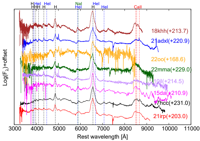
Fig. 7. Same as Figure 6, but for the late-phase spectra. The data for SNe 2010jl, 2015da, 2017hcc, and 2021irp are taken from Smith et al. (2012), Tartaglia et al. (2020), Moran et al. (2023) and Reynolds et al. (2025a).
