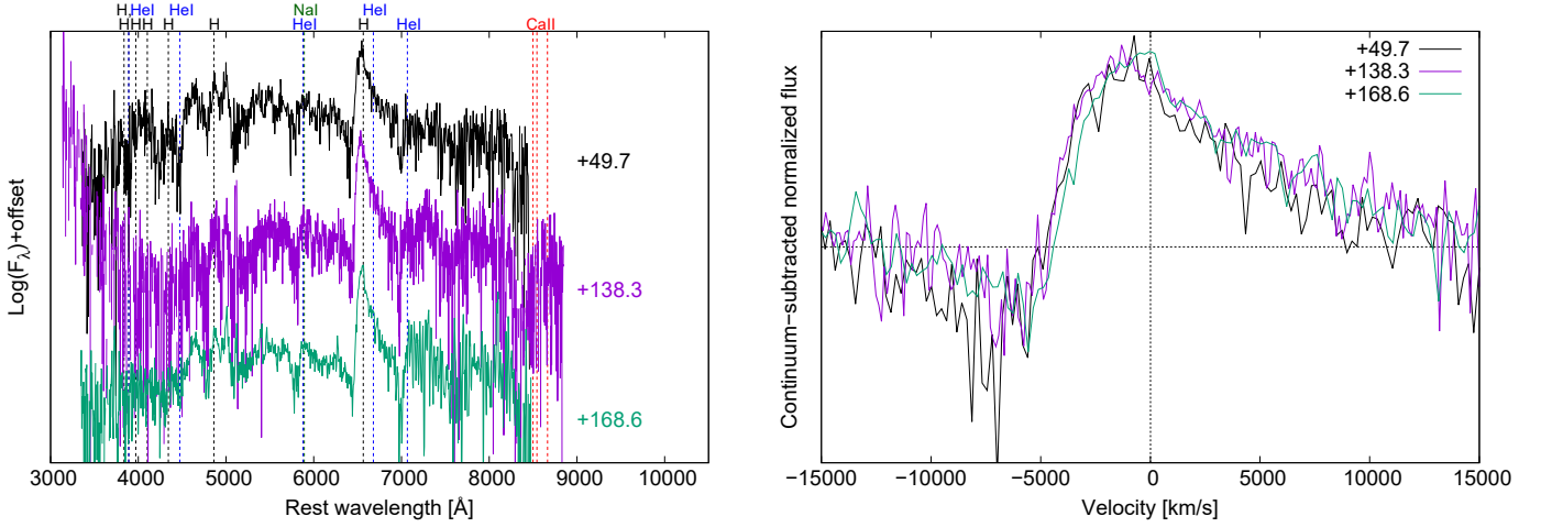
Fig. 4. Same as Fig. 2 but for SN 2022oo. The continuum level is assumed to be a constant value and estimated from the averaged value from -15\,000 to -14\,000 \text{km s}^{-1} in the velocity space.
