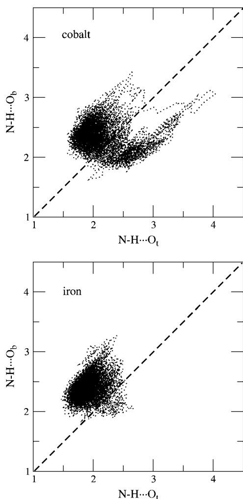
FIGURE 7 Two-dimensional distribution of the N_e\text{-H}\cdots O_t and N_e\text{-H}\cdots O_b bonds in (a) \text{FeP}(\text{Im})\text{O}_2\cdots\text{His} and (b) \text{CoP}(\text{Im})\text{O}_2\cdots\text{His} .
