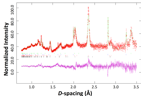
FIG. 8. Recovery run collected on a \text{Pb}(\text{Zr}_{0.54}\text{Ti}_{0.46})\text{O}_3 sample at 303 K and 0 GPa. Observed intensity is given by a red line and calculated intensity by a green line. The purple line gives the difference curve between measured and computed curves. The tick marks, from down to up, are from the R3c , Cm (due to the lower statistics of the recovery data constraints were introduced to the Cm phase so that true symmetry used in the refinements was P4mm ), NaCl, and graphite phases. The rhombohedral phase fraction was 0.633(4).
