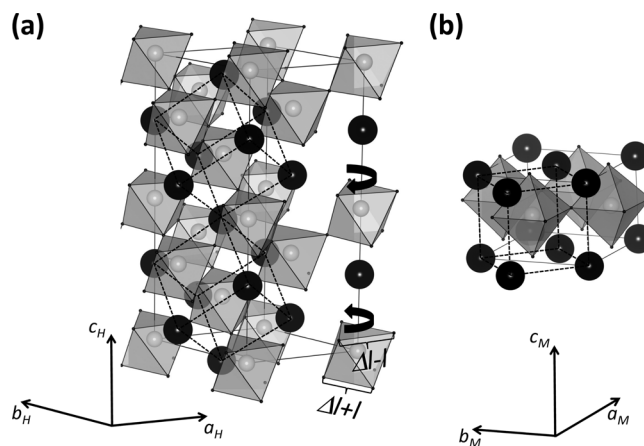
FIG. 1. The R3c phase, whose hexagonal unit cell is shown in panel (a), and the Cm phase, panel (b), behave very differently under applied pressure. The V_A/V_B ratio between the oxygen octahedral and cuboctahedra-volumes of the R3c phase decreases with increasing pressure: the crystal is contracting and thus the B cations (which fit oxygen octahedra tightly) have to take larger relative volume from the total volume (from the cuboctahedra, which has excess of space for Pb) by tilting oxygen octahedra. The symmetry prohibits this mechanism in the P4mm and Cm phases. Density-functional theory computations predict that P4mm has an entropy term benefit at elevated temperatures. Two rhombohedral (corresponding to the R3m phase) pseudocubic cells are shown by dotted lines in panel (a). Due to the octahedral tilting, indicated by arrows, the two cells are not equivalent: the tilting corresponds to the R3m \rightarrow R3c symmetry lowering. The primitive cell of the Cm phase is shown by dotted lines in panel (b). Structure figure was prepared by the VESTA software. 21
