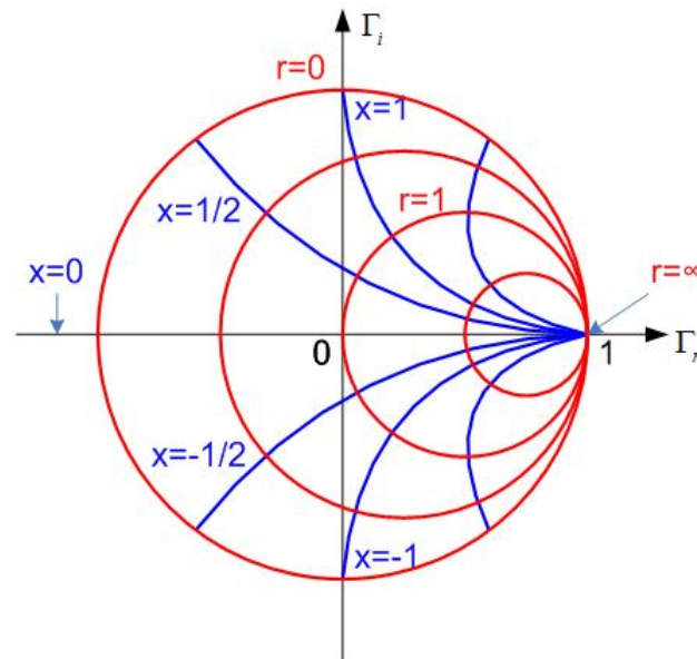
Figure 15: Smith Chart
