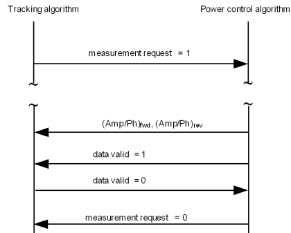
Figure 20: Interaction between tracking and power control algorithms
