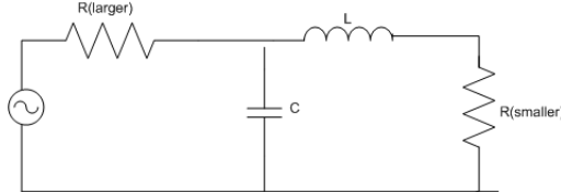
Figure 7: LC circuit (b)
