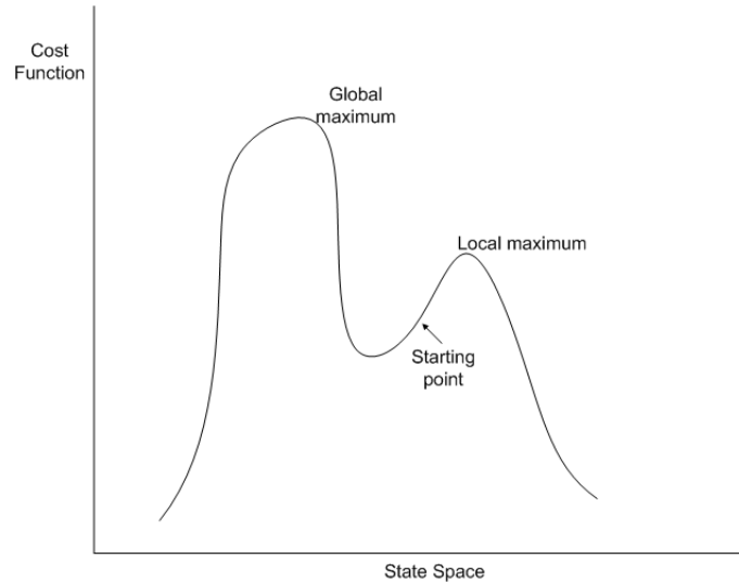
Figure 24: Hill Climbing
