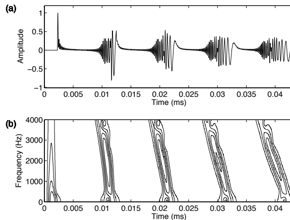
Figure 11: (a) The waveform and (b) the time-frequency plot of an inharmonic tone ( f_0 = 98.0 Hz, key G_2 , B = 0.0001 ) produced with a string model with eight first-order allpass filters in cascade. The excitation signal is simplified in order to emphasize the effect.
