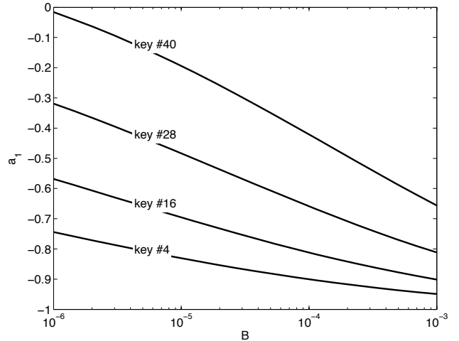
Figure 4: The dispersion filter coefficient a_1 values with B values from 10^{-6} to 10^{-3} at key indices 4, 16, 28, and 40, which correspond to keys C_1 , C_2 , C_3 , and C_4 , respectively. The number of filters in cascade M is 8 in all cases.
