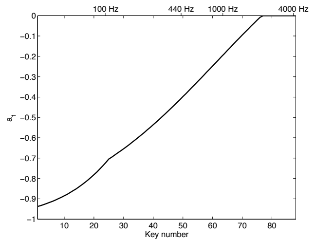
Figure 8: The dispersion filter parameter a_1 values for the piano model when a cascade of M = 8 first-order allpass filters is used.
