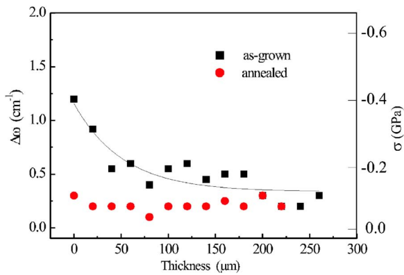
FIG. 3. Frequency shift of the E_2 mode and residual compressive in-plane stress as a function of the distance from the sapphire interface side of the as-grown and the annealed at 1350 °C HVPE-GaN freestanding films.
