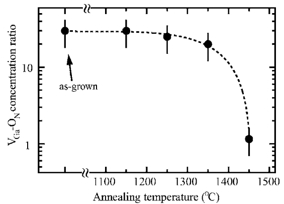
FIG. 4. V_{\text{Ga}}\text{-O}_N defect concentration ratio between N and Ga faces vs the annealing temperature of the FS GaN films.
