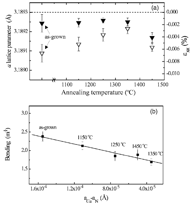
FIG. 2. (a) In-plane lattice parameters and residual strain vs annealing temperature in both sides of FS GaN films. Full symbols present the data for the Ga face, while the open symbols present the data for the N face; (b) bending vs the difference in the in-plane lattice parameters of the Ga and N face sides of the FS films.
