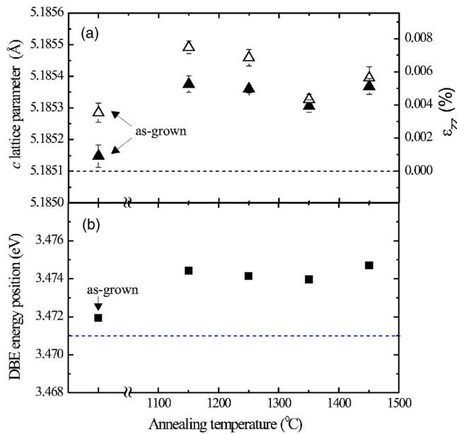
FIG. 1. (a) Out-of-plane lattice parameters and residual strain in growth direction vs annealing temperature in both sides of FS GaN films. (b) Energy position of the DBE line in 2K PL spectra vs the annealing temperature determined in the as-grown (Ga face) side of the FS films. Full symbols present the data for the Ga face, while the open symbols present the data for the N face. The dashed lines indicate the strain free positions for the respective parameters.
