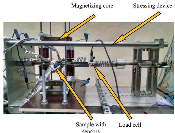
Fig. 1. Experimental setup for measuring unidirectional magnetization curves under stresses parallel to the magnetic field.
