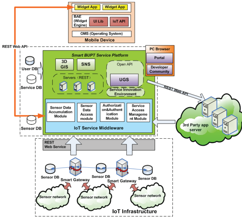
Figure 5. Smart BUPT architecture
