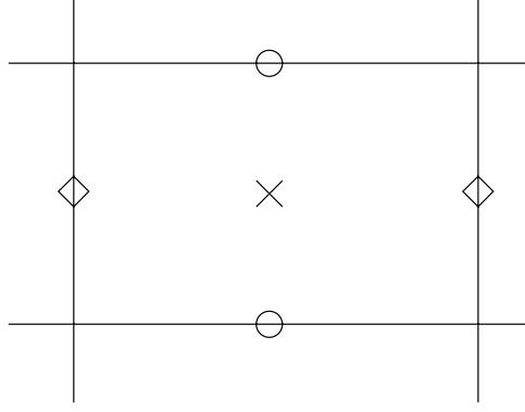
Figure 2: Finite difference approximation of the shear and membrane constraints in the reduced-strain FE formulation: \rho_1 = \beta_{11} = 0 at ( \odot ), \rho_2 = \beta_{22} = 0 at ( \diamond ) and \beta_{12} = 0 at ( \times ).
