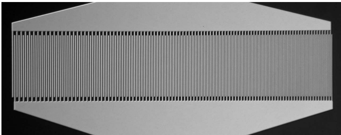
Figure 3.12: Photograph of the chirp transducer of the UWB SAW tag shown in Fig. 3.11. The low-frequency sections are on the left and the high-frequency sections on the right. The transducer length is 400 \mu\text{m} and aperture 75 \mu\text{m} .
