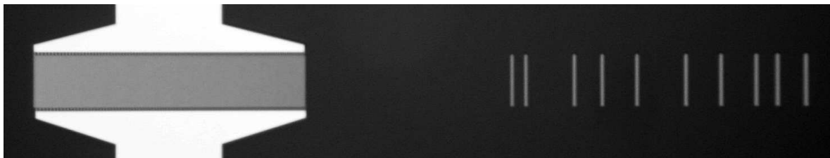
Figure 3.11: Photograph (taken through a microscope) of the fabricated UWB SAW tag device. The length of the structure is 1.1 mm.
