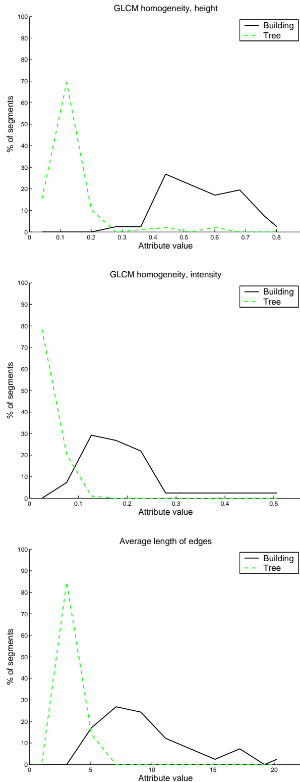
Figure 1. Histograms of attribute values for building segments and tree segments.
