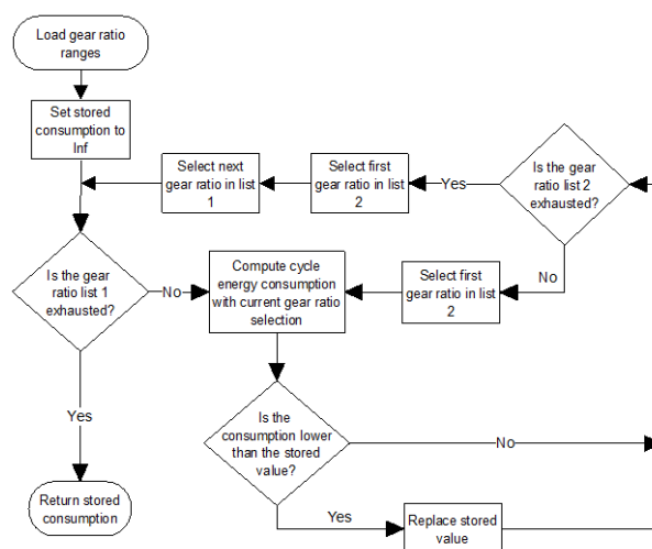
Figure 3. Flow chart of the gear ratio optimization process.
