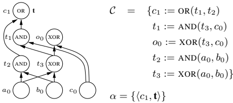
Figure 1. A constrained Boolean circuit \mathcal{C}^\alpha .
