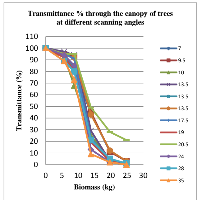
Figure 6. Transmittance through the canopy of trees at different scanning angles (from 7 to 35 degrees). We stratified the scanning angles into three parts at each height. The angle value presented is the mean value of each part.
