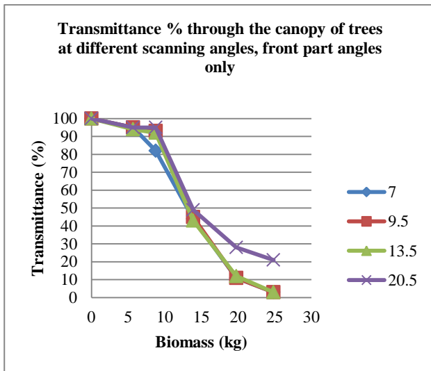
Figure 7. Transmittance through the canopy of trees at different scanning angles. Only the front part angles are presented for each scanning height (9, 7, 5 and 3 m).
