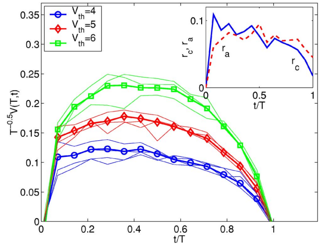
FIG. 2. (Color online) The average scaled avalanche shape for different threshold values V_{th} for \sigma=0.03 and L=300b . For small threshold values the avalanches are asymmetric with the asymmetry decreasing with V_{th} . The thick lines with circular symbols correspond to an average over of the order of 10^3 avalanches, which have been scaled according to Eq. (5) before averaging. The thin solid lines correspond to avalanches of different limited duration ranges. The inset displays the average creation and annihilation rates ( r_c and r_a , respectively) of dislocations during an avalanche, with V_{th}=5 .
