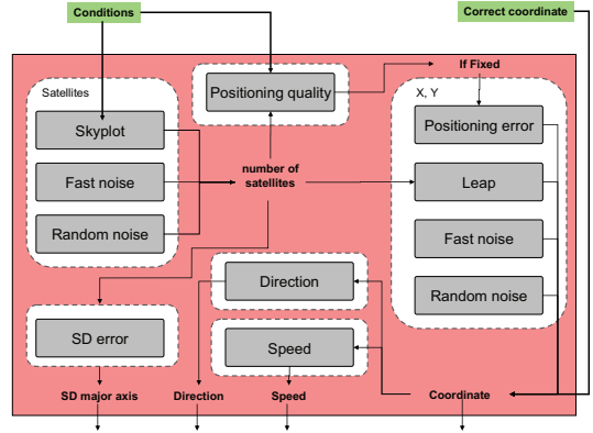
Figure 4. The structure of the GPS-noise model
