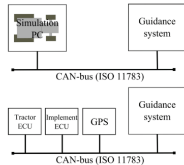
Figure 2. The simulation environment and the real system
