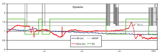
Figure 1. HDOP, the number of SVs and the accuracy.
