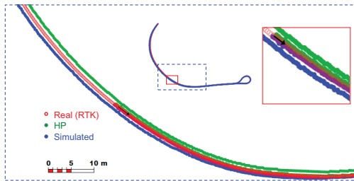
Figure 7. The recorded trajectory of the real vehicle and the simulated trajectory with the same control values.
