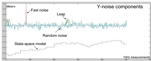
Figure 5. Y-axis errors caused by different components.
