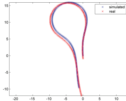
Figure 6. The recorded trajectory of the real vehicle and the simulated trajectory with the same control values.
