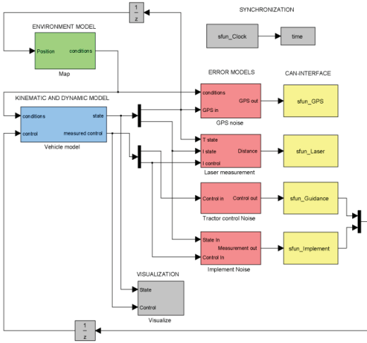
Figure 3. The overall structure of the simulator in Matlab Simulink - environment.
