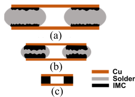
Fig. 1. Schematic of (a) FC bumps with diameter D \approx 100 \mu\text{m} and (b) with D \approx 30 \mu\text{m} , and (c) SLID bumps with D < 30 \mu\text{m} .
