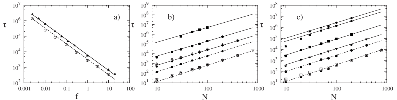
FIG. 2. (a) The scaling of the translocation time \tau with respect to the external force f . Results from two dimensions ( \blacktriangle ) and three dimensions ( \circ ) Langevin dynamics simulations yield the same f \sim N^{-1} scaling. Since the simulations were done with the only difference in dimension, we note that in higher dimension the translocation process is faster. (b) 2D and (c) 3D Langevin dynamics simulation results for the scaling of the translocation time \tau with respect to chain length N with various forces. Open symbols are with frictional pore and full symbols are with a ballistic pore. All plots yield different values for the scaling exponent \beta which are reported in Table I along with their corresponding forces. The finite size effect due to the frictional is identical to the 1D case (see text). With f=10 only chains with N \geq 200 follow the asymptotic scaling behavior. If the pore is nonaqueous (i.e., ballistic) the finite size effect applies only for chains smaller than N=30 , and is amplified by reducing the force.
