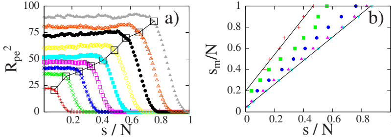
FIG. 6. (Color online) (a) 3D Langevin dynamics. Averaged squared distances of beads numbered 30, 50, 70, 100, 200, and 400 from the pore as a function of the number of translocated beads s for polymers of length N=100 . The force f=0.25 . (b) The number of mobile beads s_m vs the number of translocated beads s , both normalized to the polymer length N .
