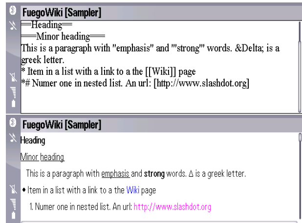
Figure 6: Editor and formatted views for an article.
