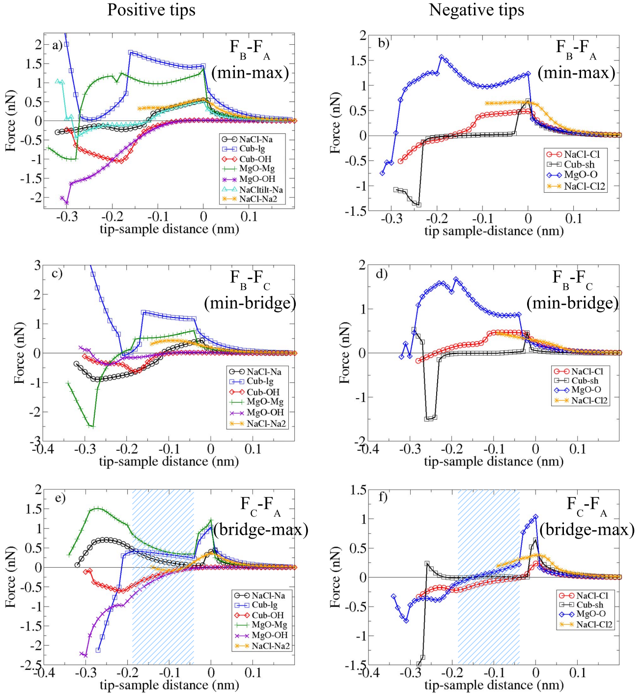
FIG. 6. (Color online) Calculated force difference curves: F_B - F_A for tips with strongest attraction to (a) surface anions and (b) surface cations; F_B - F_C for tips with strongest attraction to (c) surface anions and (d) surface cations; F_C - F_A for tips with strongest attraction to (e) surface anions and (f) surface cations where A is the topographical maximum, B the minimum and C the bridge site. All x axes of the curves have been normalized so that zero is at the position of the first maximum in the minimum-maximum curves. The hatch shows the region where a nearly linear slope is observed. This slope is characteristic for the tip termination for all tips except the OH-terminated tips. The z axes of all models are normalized such that the maxima in the min-max curve match and are set to 0.
