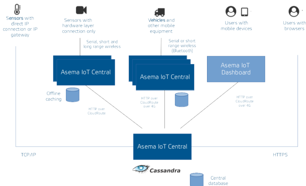
Figure 4.1: Asema IoT Solution High-level Architecture [39]
