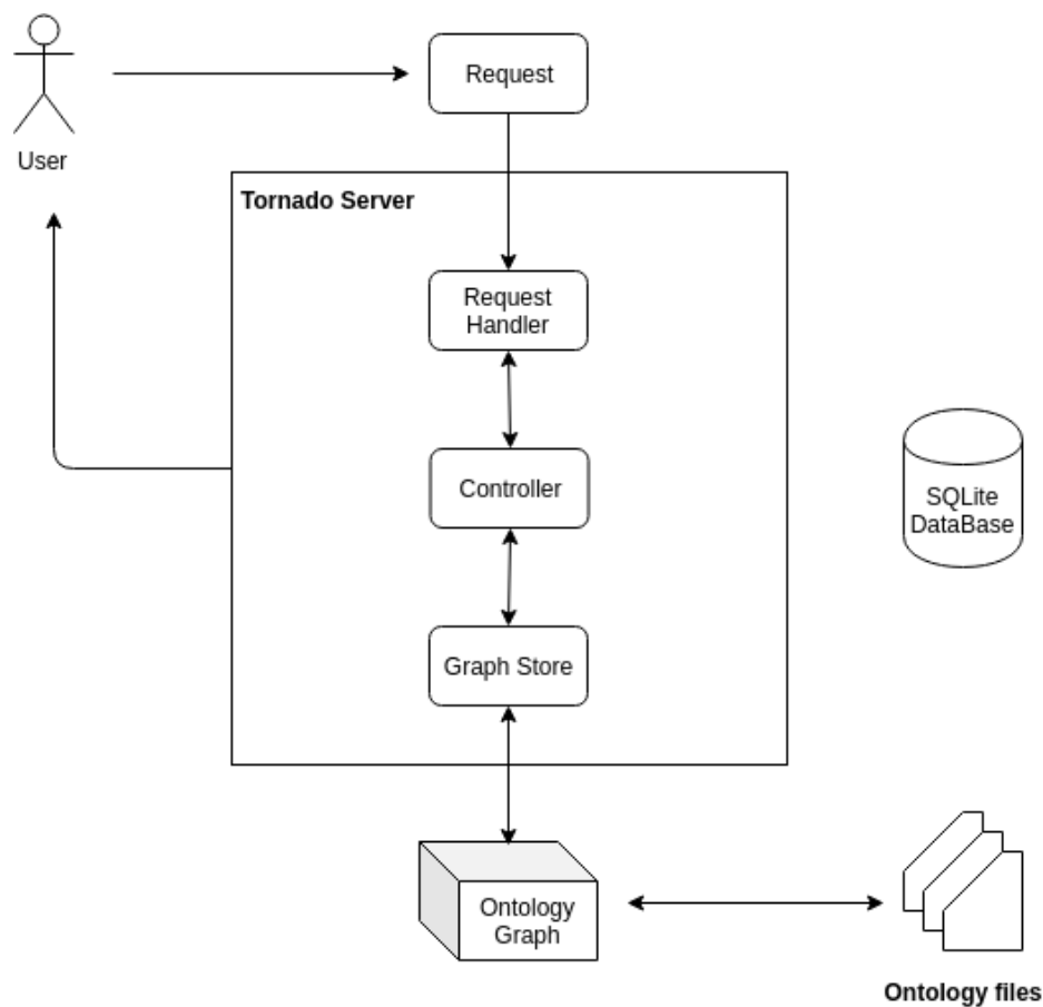
Figure 4.14: Backend Architecture
