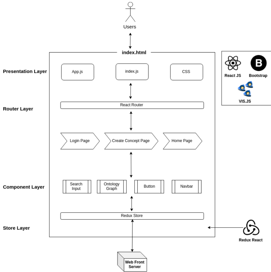
Figure 4.13: Frontend Architecture
