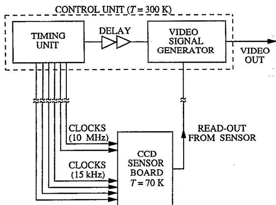
FIG. 1. Principal scheme of the remote-controlled CCD imager.
