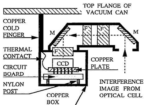
FIG. 2. Mounting of the CCD sensor inside the 4 K vacuum can. Cables connecting the circuit board to the control unit are not shown. F=thermal filter, M=mirror.
