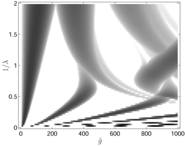
FIG. 1. Grayscale plot of the maximum imaginary part of the Bogoliubov eigenvalues as a function of the interaction strength \tilde{g}=4\pi aN/a_r and inverse trap anisotropy 1/\lambda=\omega_r/\omega_z for the two-quantum vortex state. White denotes the dynamically stable regions with vanishing imaginary parts, and black corresponds to maximum imaginary part 0.185\omega_r , the scale in between being linear. The strip-like instability regions for small 1/\lambda are in fact continuous, although they seem fragmentary due to discretization of the parameter space in the computations.
