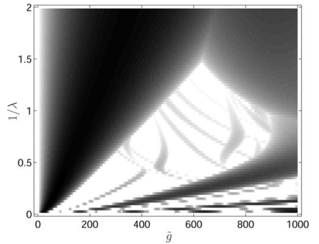
FIG. 3. Maximum imaginary part of the Bogoliubov eigenvalues as a function of the interaction strength \tilde{g}=4\pi aN/a_r and inverse trap anisotropy 1/\lambda for the three-quantum vortex state. In the grayscale white corresponds to dynamically stable state and black the imaginary part value 0.208\omega_r of the frequency. The large instability regions are due to modes with \kappa_q=2 , and the thin lines in between them are caused by modes with \kappa_q=3 .
