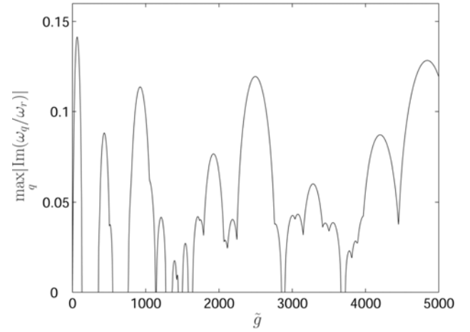
FIG. 2. Maximum imaginary part of the Bogoliubov eigenvalues for the two-quantum vortex state as a function of the interaction strength \tilde{g}=4\pi aN/a_r for the spherically symmetric trap geometry with \lambda=1 .
