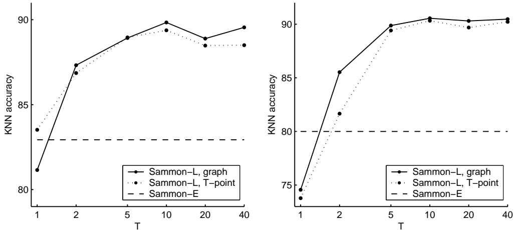
Fig. 7. The KNN-classification accuracy of Sammon-L mapping increases rather quickly with the distance parameter T on both the Landsat (left) and Phoneme (right) data sets. The difference to Sammon-E performance is clear already with T = 2 and using values larger than T = 5 seems unnecessary. The local approximation ( T = 1 ) is not sufficient, as was to be expected.
