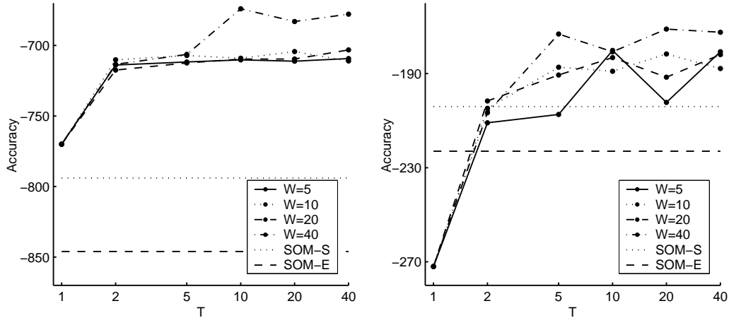
Fig. 6. SOM accuracy for Landsat (left) and Phoneme (right) data as a function of the computational complexity. The effect of the speedup parameter W is not altogether clear, but in general the larger W work better. On the Landsat data the SOM-L results are always better than the comparison methods (SOM-S and SOM-E), but on the Phoneme data the least accurate approximations are not accurate enough.
