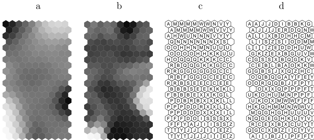
Fig. 1. Sample SOM-L visualizations for Letter Recognition data. (a) The component plane showing, with gray shades, the values of one of the components (called “height of the centroid of mass”) in the map units, and (b) the importance of the component. The map has been computed with the T -point distance approximation and the units have been labeled by majority voting (c). The feature has a high importance (light shade; large contribution to the local distance) on two separate regions of the map. One region corresponds to the letter “L” and the other to the letter “T”. The component plane reveals that in “L” the mass centroid is low whereas in “T” it is high. The majority voting on SOM-E (d) is given for comparison; the labels are clearly more dispersed on the map compared to the SOM-L.
