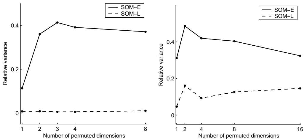
Fig. 5. Effect of irrelevant variation on SOM-L, measured by variances of model vectors along permuted dimensions relative to variances in the original data. Solid line: SOM-E, dashed: SOM-L.
