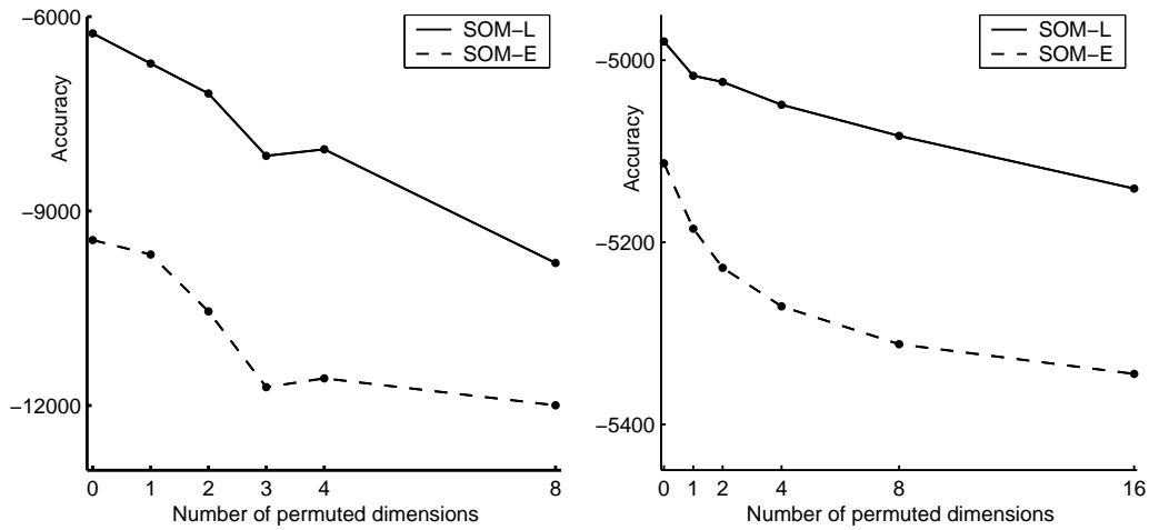
Fig. 4. Replacing interesting with uninteresting variation decreases the accuracy of both SOM-L and SOM-E at a similar rate. On the Letter Recognition data (left), even when half of the dimensions are permuted, SOM-L performs as well as the SOM-E for the original (unpermuted) data. On the gene data (right) permuting roughly 10 out of 42 dimensions reduces the SOM-L performance to the level of a SOM-E for original data.
