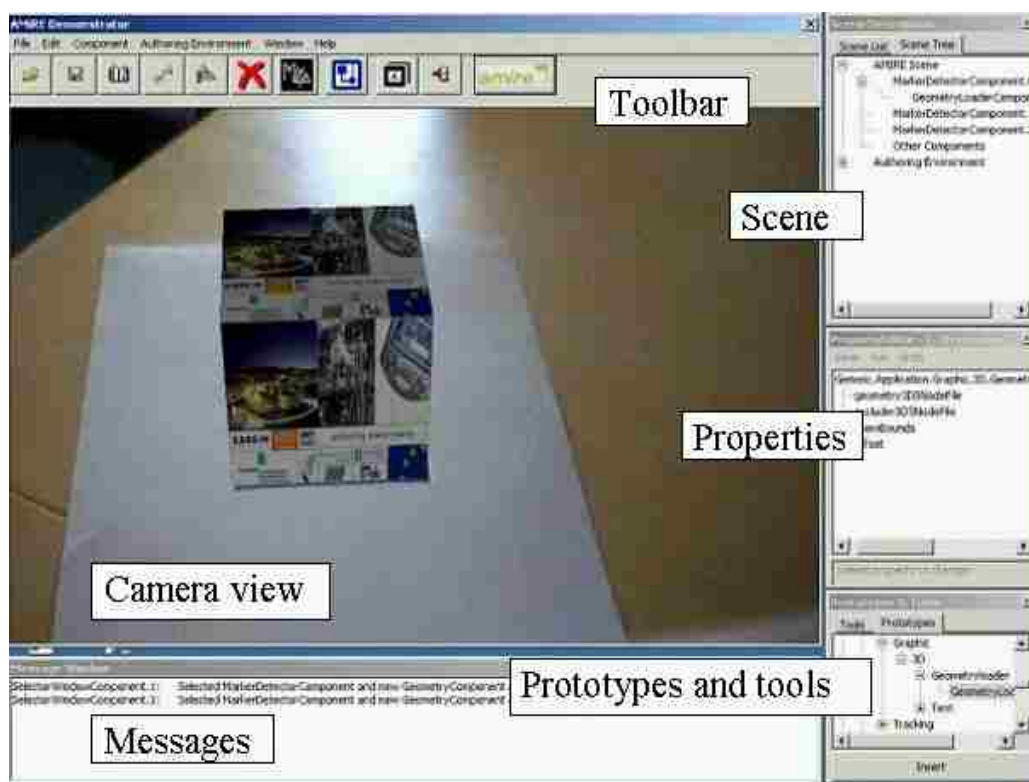
Figure 9. The user interface of the AMIRE authoring tool
