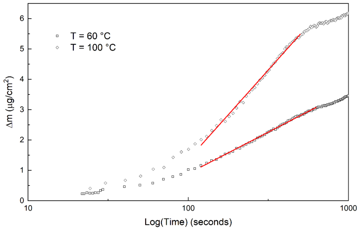
Figure 5. Examples of determination of the logarithmic rate constants at 60 °C and 100 °C.
