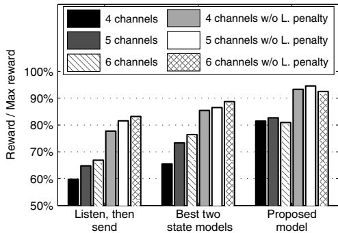
Fig. 2. Tests with dynamic HTTP+VOIP traffic. Total reward and total reward without listen collision penalties, divided by the maximum reward possible (4365000) for our proposed model, the best two state models, and the simple randomized listen-then-send model. Results of the proposed model on 6 channels are initial results from brief training, which already worked well.
