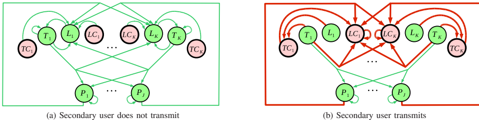
Fig. 1. State transitions for one channel in our model. Transitions depend on whether the secondary user (SU) chooses to transmit on this channel (b) or not (a). The primary user (PU) can transmit K types of packet bursts and have J types of pauses. In normal operation, each packet burst i starts with a listen state L_i , continues with transmit state T_i for some amount of steps, and then the channel moves to a pause state or to the listen state of another packet burst; similarly, each pause state P_j lasts for some amount of steps and then the channel moves to a listen state of a packet burst. If the SU starts transmitting when the PU is about to listen or transmit, the channel moves to listen collision state LC_i or transmit collision state TC_i respectively. Collision states and transitions to them are shown with red color and thick lines. After collision, the PU listens until the SU does not transmit, then reattempts normal operation.
