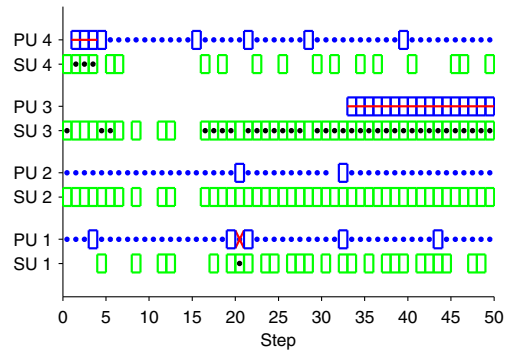
Fig. 3. Example of our proposed model on 4 channels, each with its own primary user (PU). One secondary user (SU) operates over the channels. For the SU and each PU, empty boxes denote sensing; dots denote transmissions; boxes with horizontal lines are listen collisions; dots with crosses are transmit collisions. The shown 50 steps were chosen from a test segment with 20 listen collisions, to show they are harder to avoid than transmit collisions.
