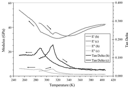
Fig. 1. DMA measurement curves of the sample A1 as a function of temperature.
