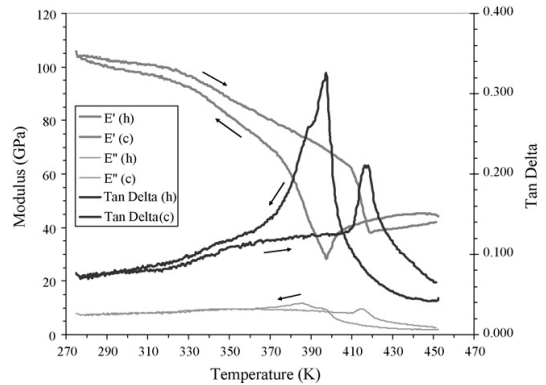
Fig. 4. DMA measurement curves of the sample A4 as a function of temperature.
