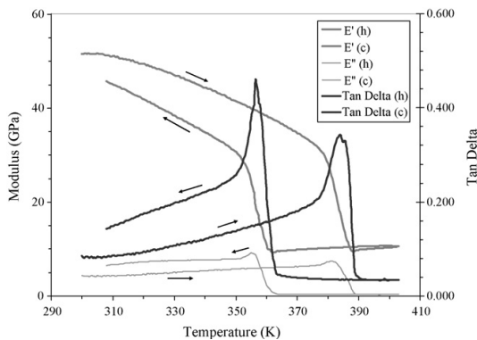
Fig. 3. DMA measurement curves of the sample A3 as a function of temperature.
