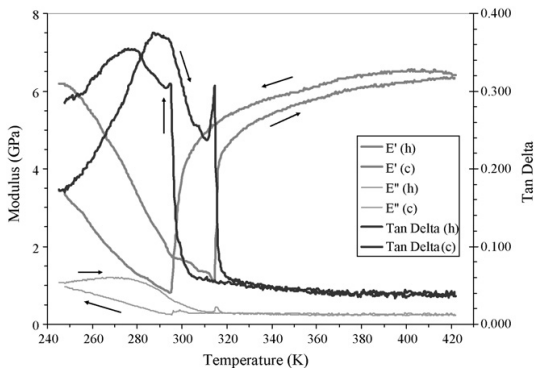
Fig. 2. DMA measurement curves of the sample A2 as a function of temperature.
