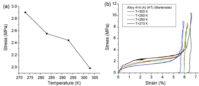
Fig. 5. Twinning stress of A1 (in H=0 ) determined from the 4.5% strain at different temperatures (left) and the corresponding compression \sigma - \epsilon -curves (right).
