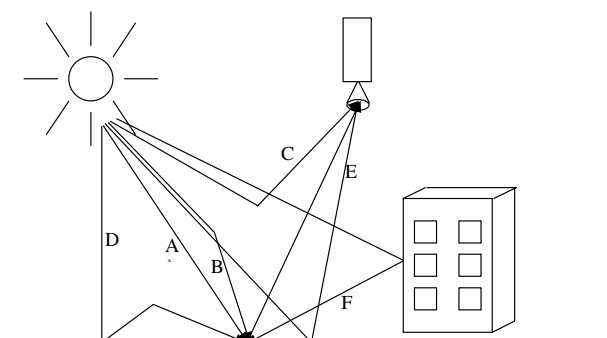
Figure 6. Radiation components (adopted from Beisl 2001).
