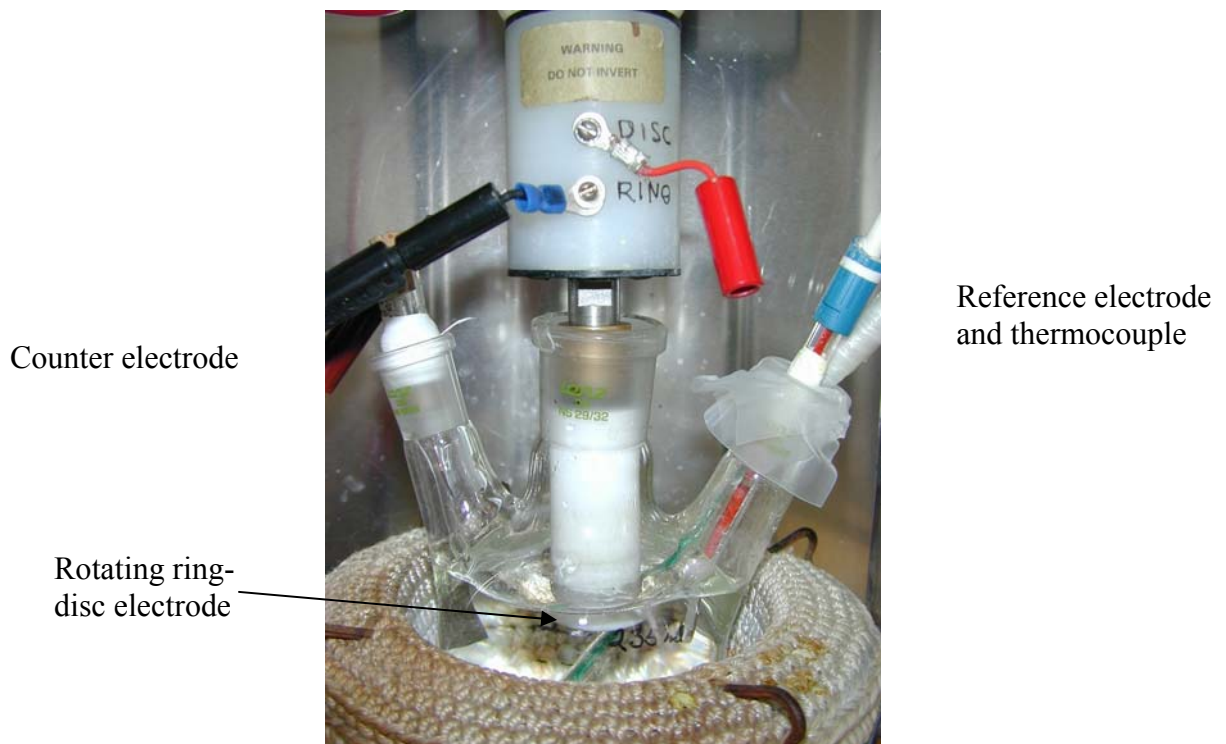
Figure 20. A picture of the RRDE-equipment.
