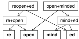
Figure 1: Hypothetical binary splitting trees for the words reopened and openminded (segmented as “re+open+ed” and “open+mind+ed”). The leaf nodes of the trees correspond to morphs discovered by the algorithm.
