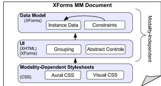
Figure 2: The XFormsMM Authoring Format.
